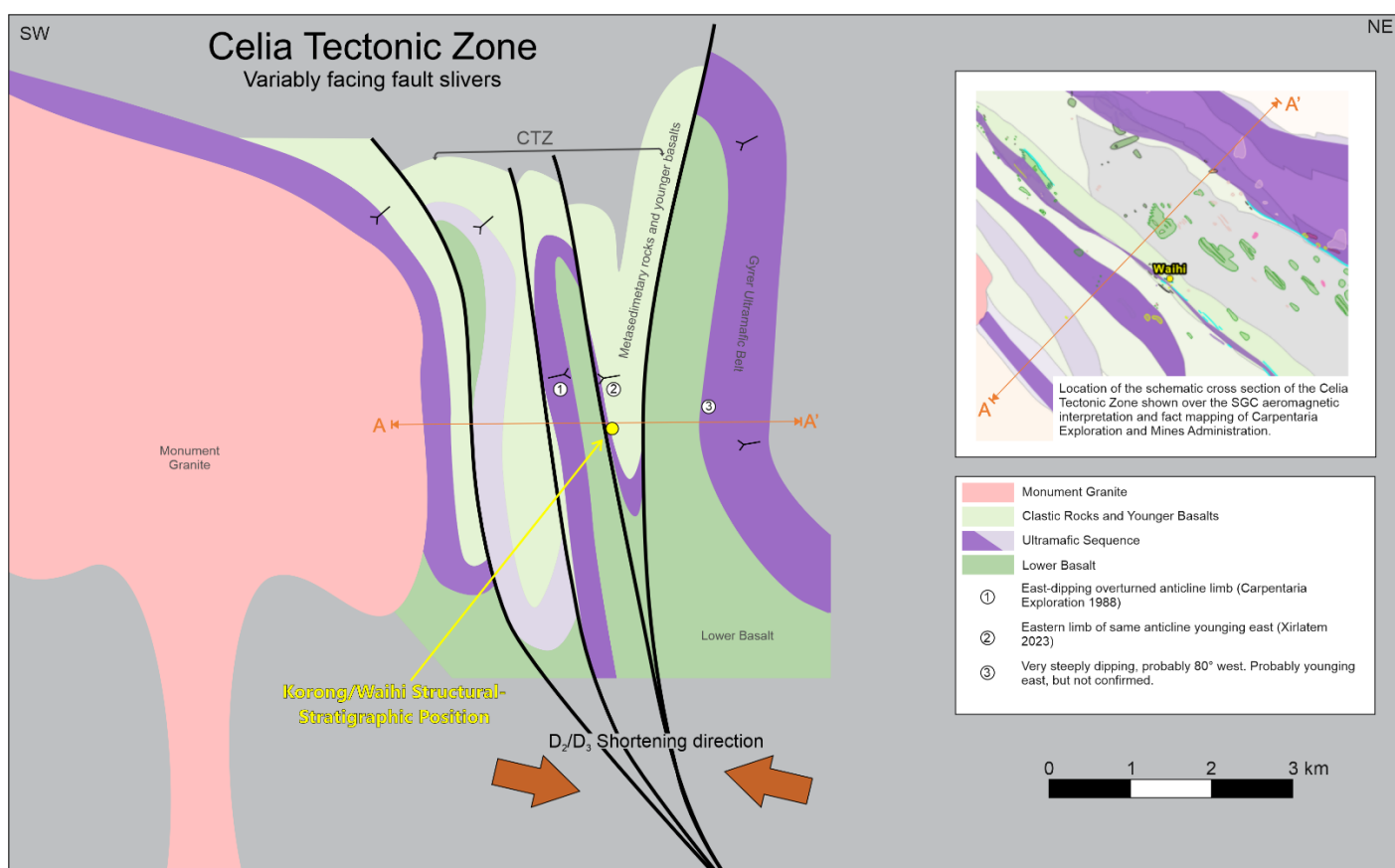
Figure 1. A schematic cross section of the regional setting of Korong and Waihi with respect to the Celia Tectonic Zone.
