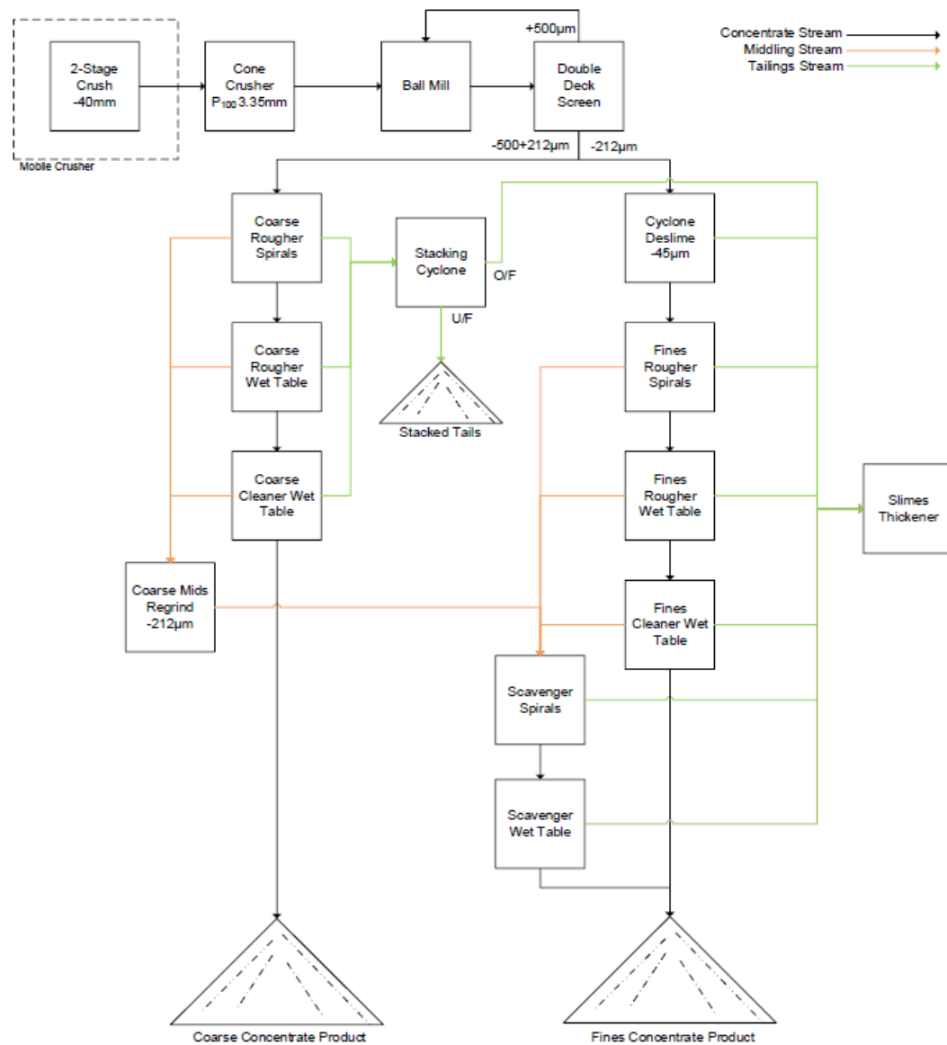
Figure 3 – Tabbatabba Resource Process Flow Block Flow Diagram
