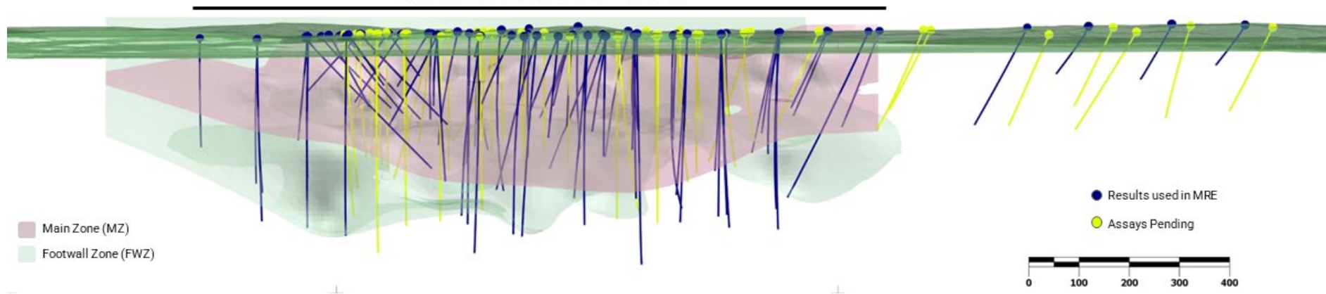
Figure 1. Long Section of Main Zone showing conceptual pegmatite model showing strike extent of systematic drilling and extensions to mineralisation defined to the east.
