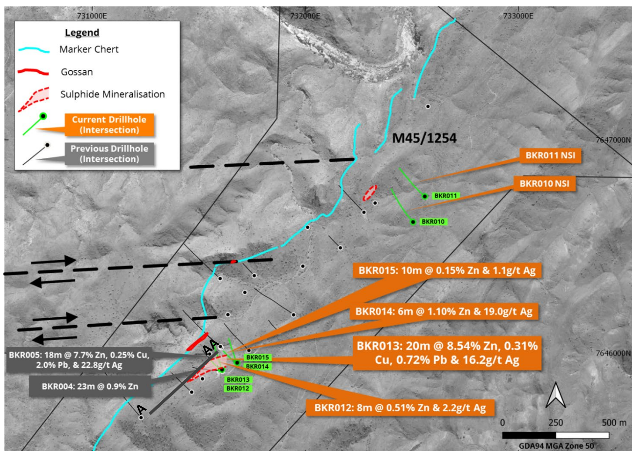
Figure 1: Plan view of Breakers exploration drilling.
